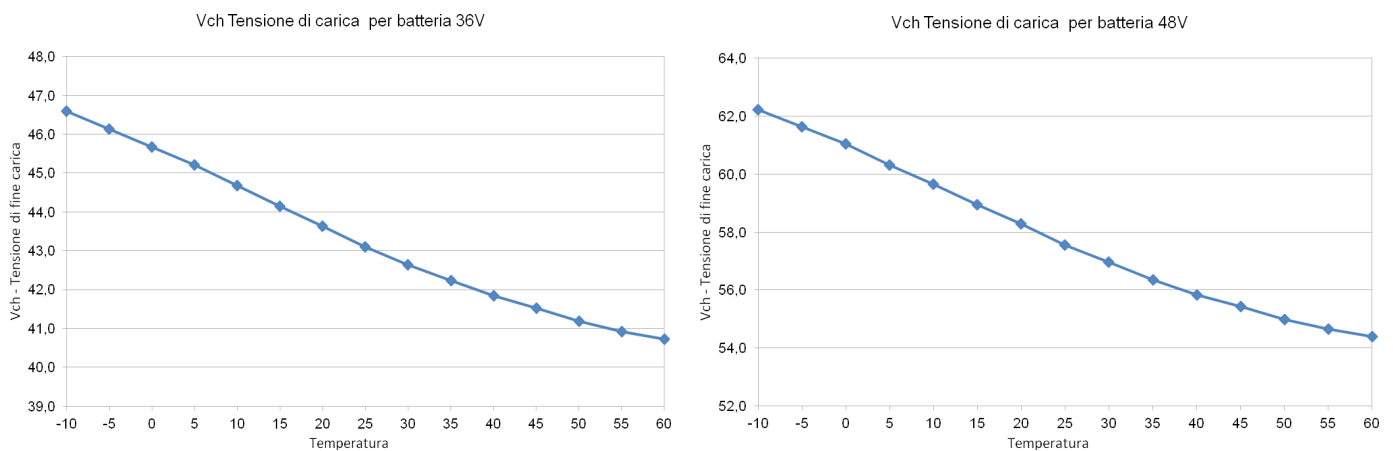
Fig.3 End of charge current for lead acid batteries.
